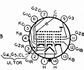
14AU ULTOR = G_4 + G_5 + CL FOCUSING ELECTRODE = G_3
